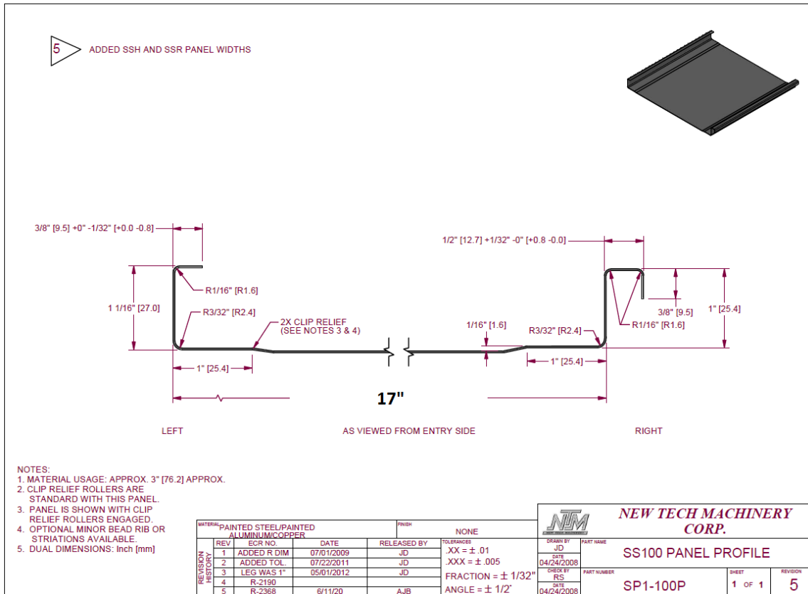
Drawing # 2 Panel Dimensions
